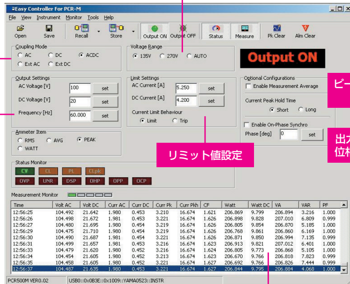
▲ Easy Controller For PCR-M
